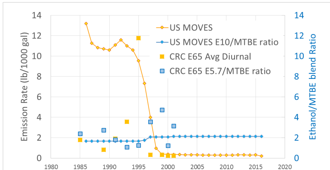
Figure 14: Improvements in Permeation Emissions over Time
