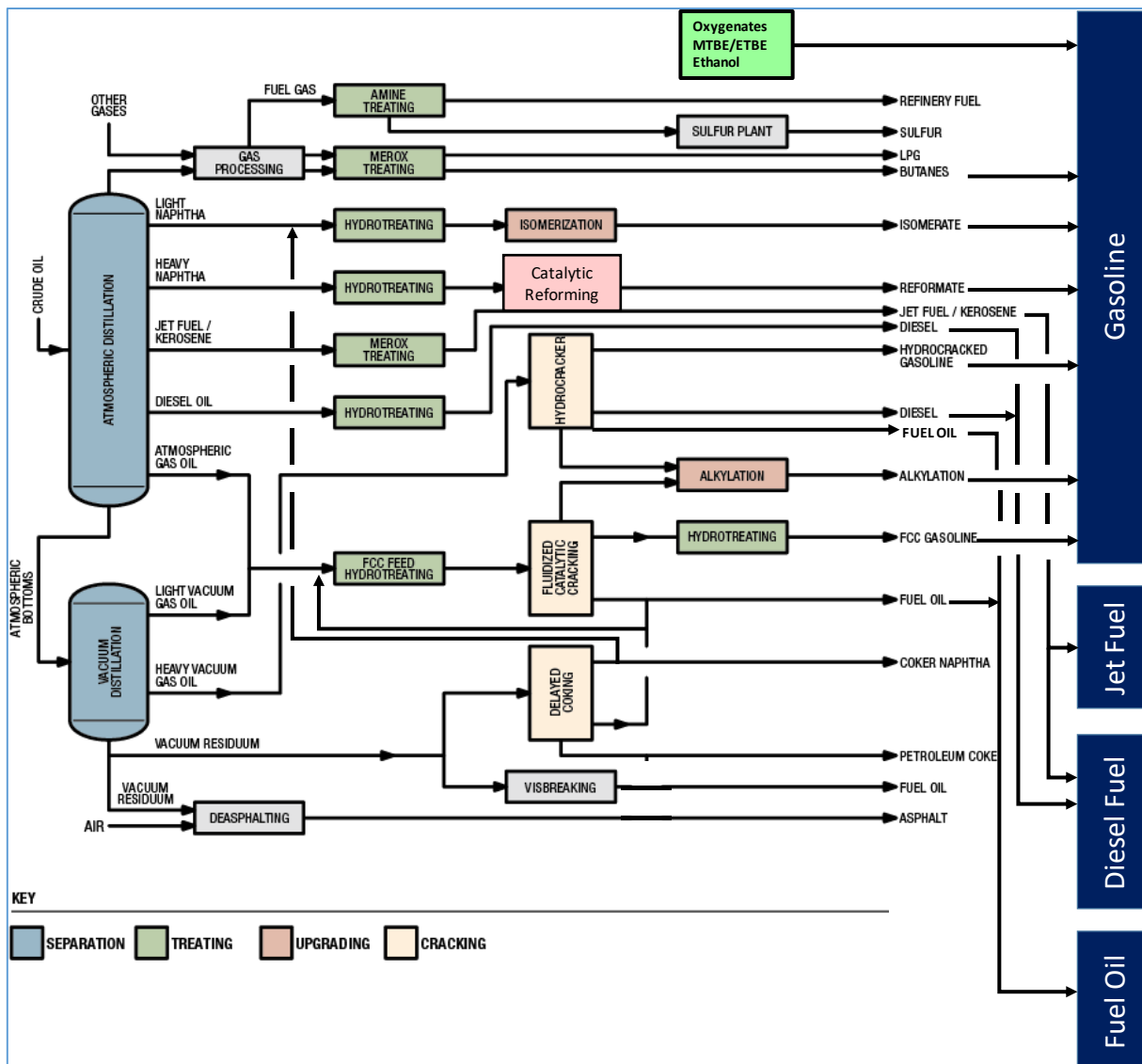
Figure 18: Refinery Schematic
