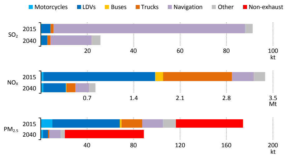
Figure 6.5 ▶ Air pollutant emissions by transport type in the European Union in the New Policies Scenario
