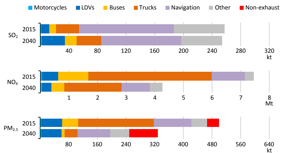
Figure 7.7 ▶ Air pollutant emissions by transport type in China in the New Policies Scenario
