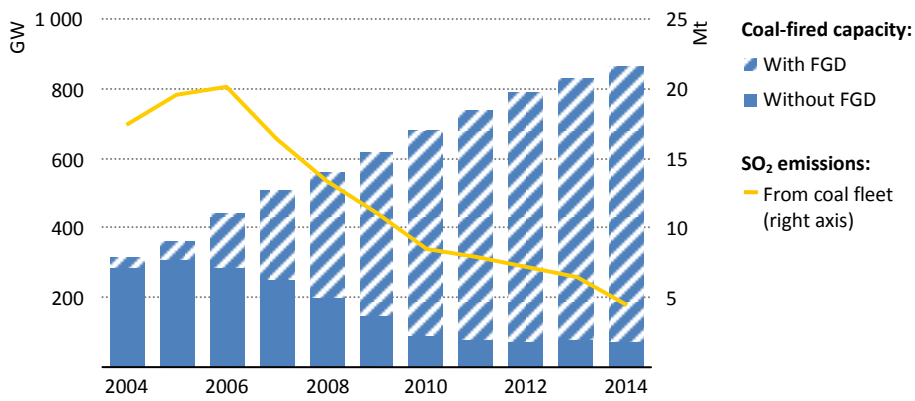
Figure 7.3 ▶ Coal power capacity equipped with flue-gas desulfurisation and related SO 2 emissions in China
