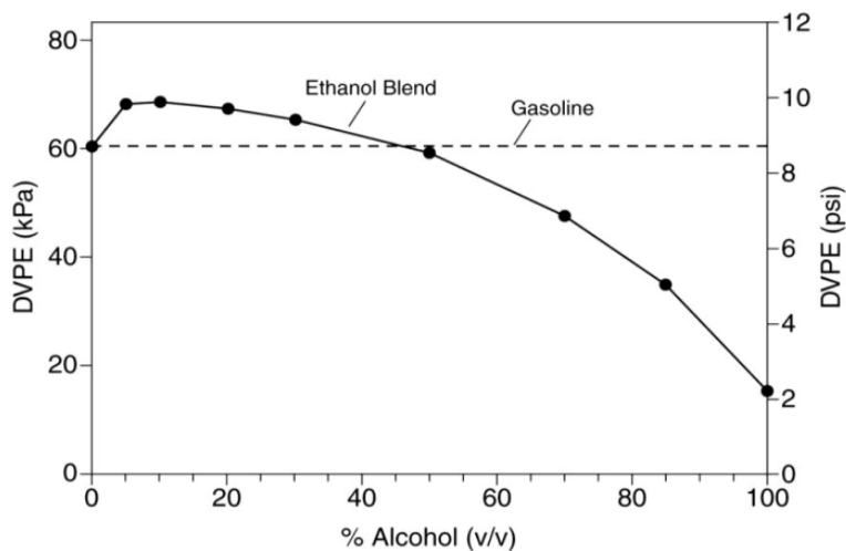
FIGURE IV-5 Effect of Ethanol Blending on Gasoline Vapor Pressure
