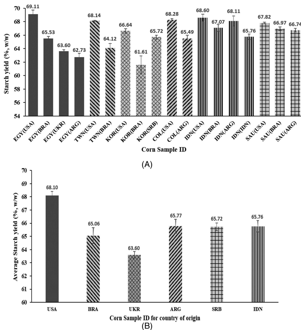
Figure 1. Wet mill starch yield comparison of commodity corn. a) Starch yield (% w/w) of individual samples. b) Average starch yield (% w/w) of the samples from a particular origin. Corn sample IDs represent the corn exported from the United States of America (USA), Brazil (BRA), Ukraine (UKR), Argentina (ARG), Serbia (SRB) to the countries of export Egypt (EGY), Taiwan (TWN), South Korea (KOR), Colombia (COL), Indonesia (IDN), and Saudi Arabia (SAU).
