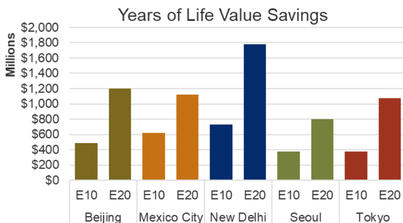
Figure 3: Summary of Years of Life Value Savings by City and Ethanol Blend
