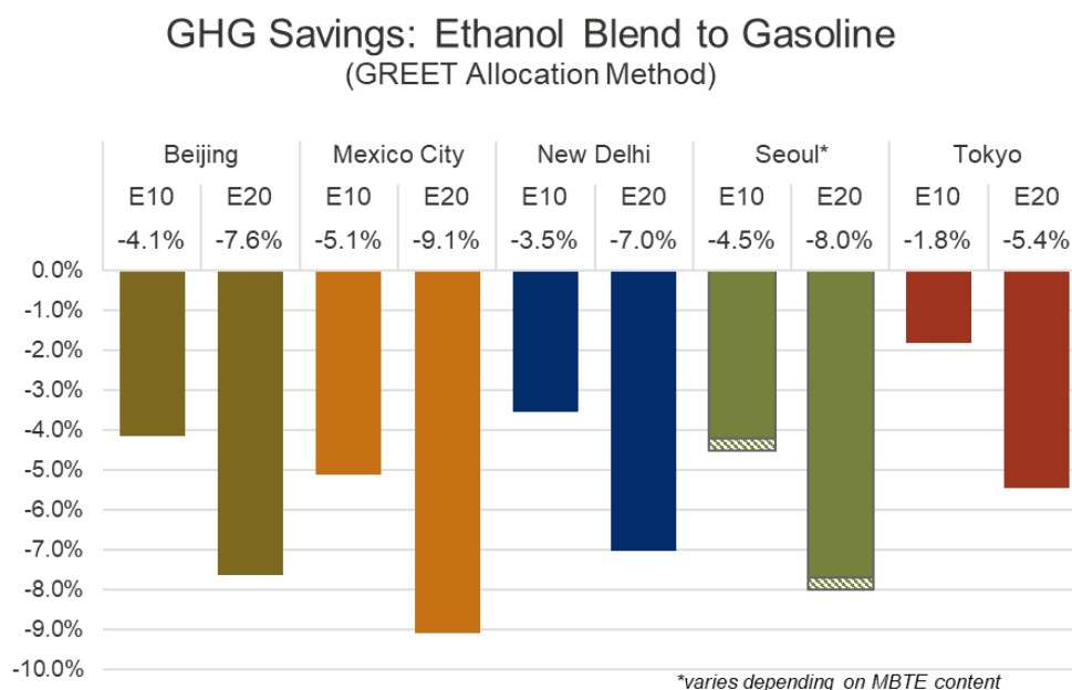
Figure 3: Cumulative GHG Savings by City and Blend
