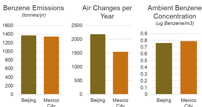
Figure 14: Box Model Relating Mass Emissions to Concentrations
