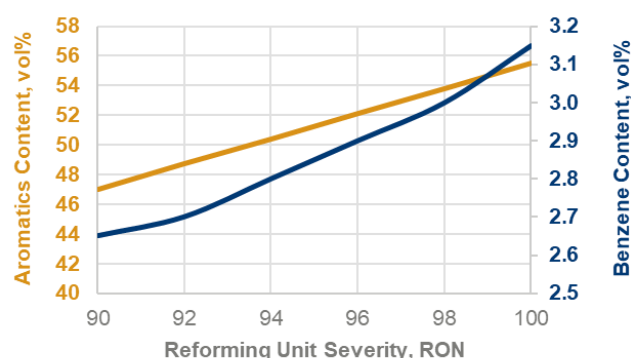
Figure 12: Aromatics Production at Refinery to Meet Octane Requirements
